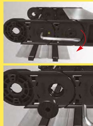
Easy opening of the pin junction.
