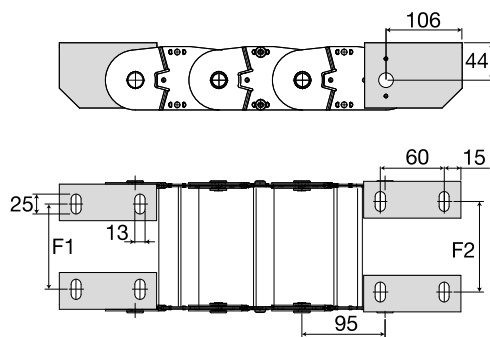
Fig. A Chain fixed outer radius. (Fig A)
